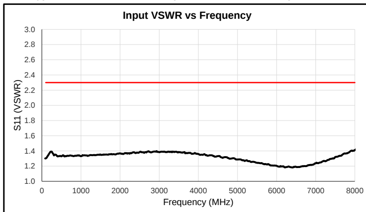
Typical Performance @ 23°C (Reference S/N 2162303)
